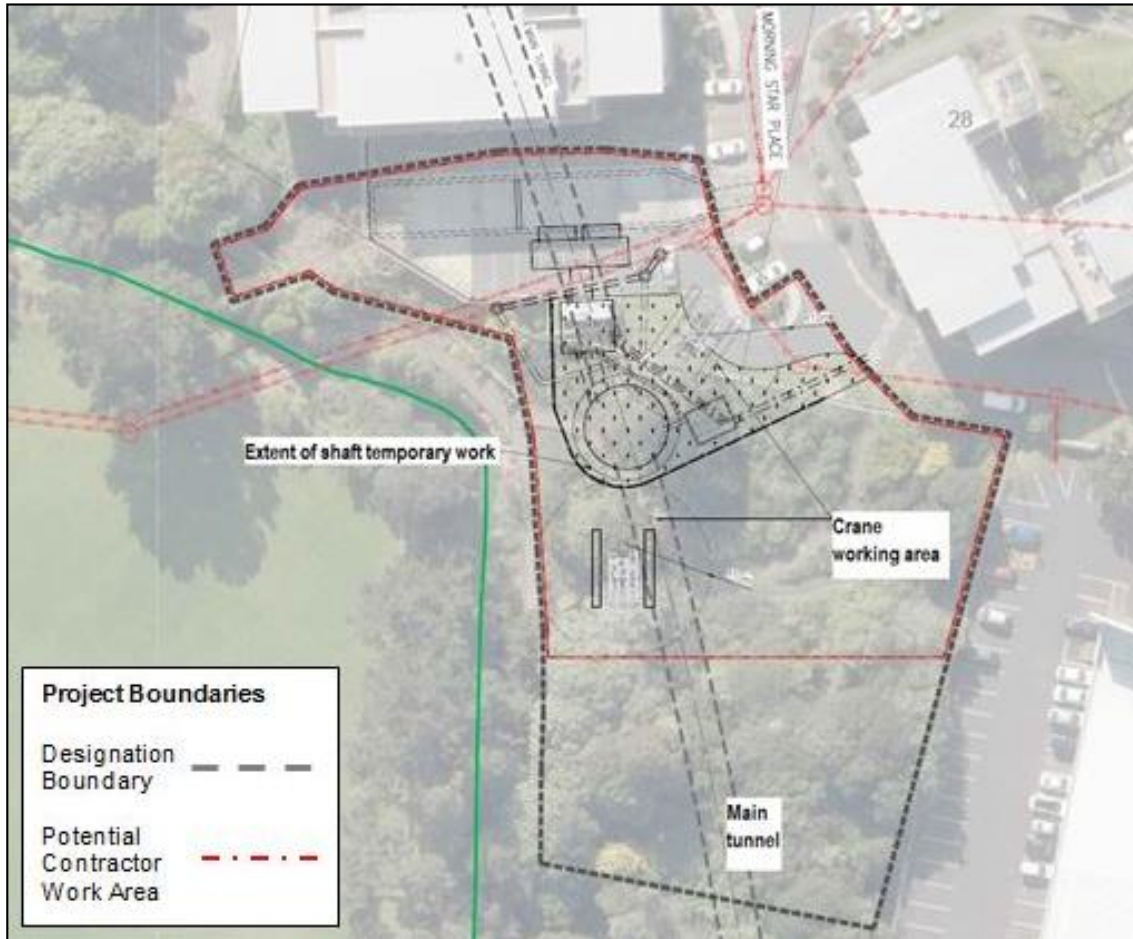
Figure 1 Overview of the Lyon Avenue construction site
