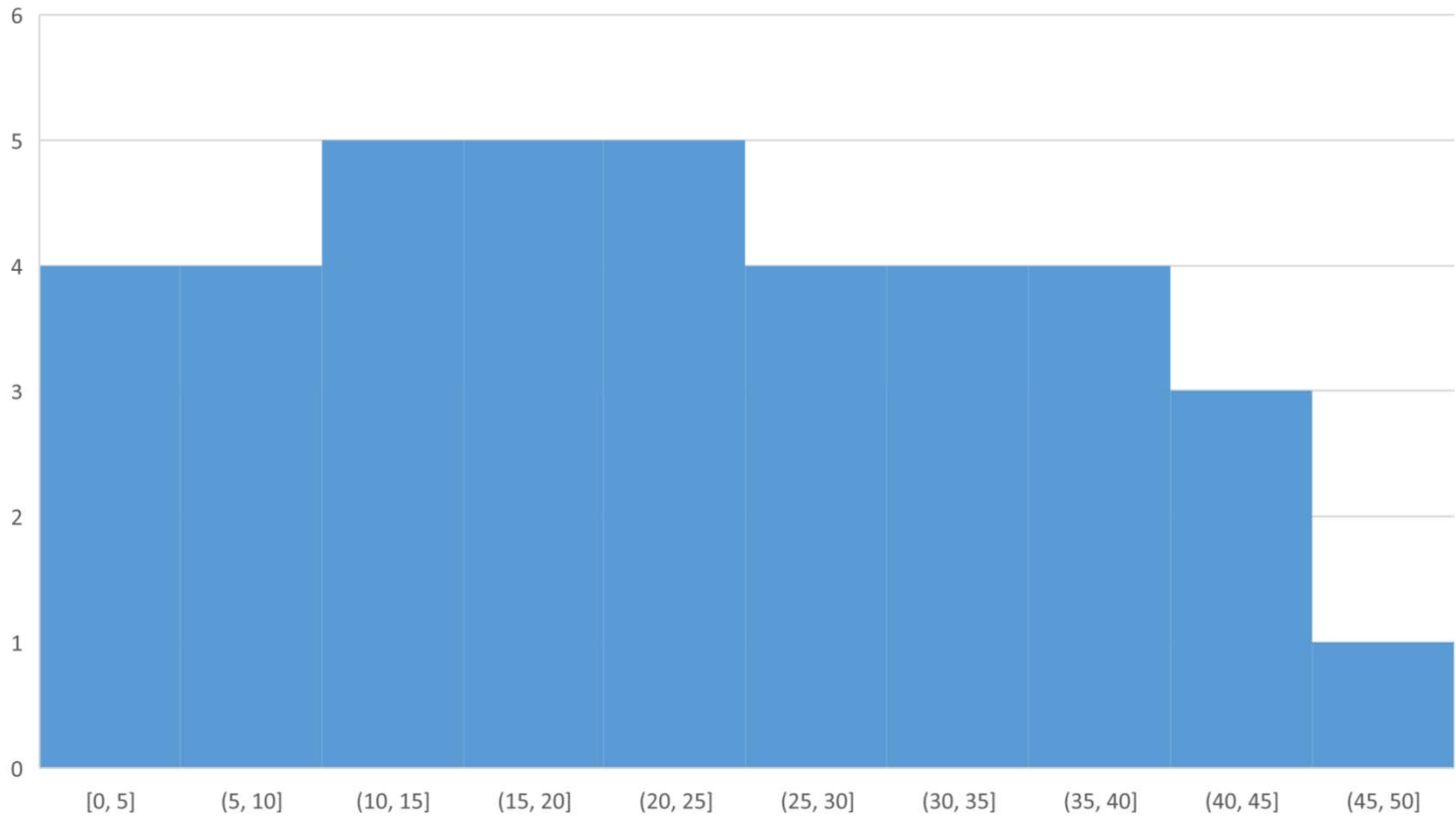
Score distribution
